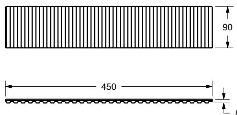
Figure 3 – Isolator pads
